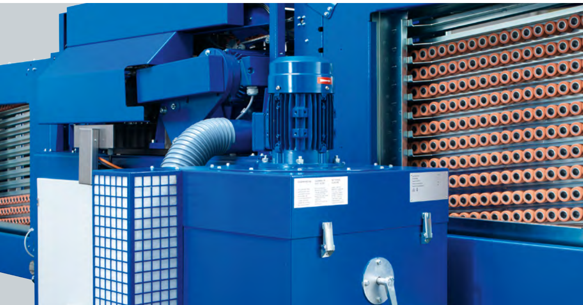
supergrinder view from the back with supplied suction device and large universal loading magazine
